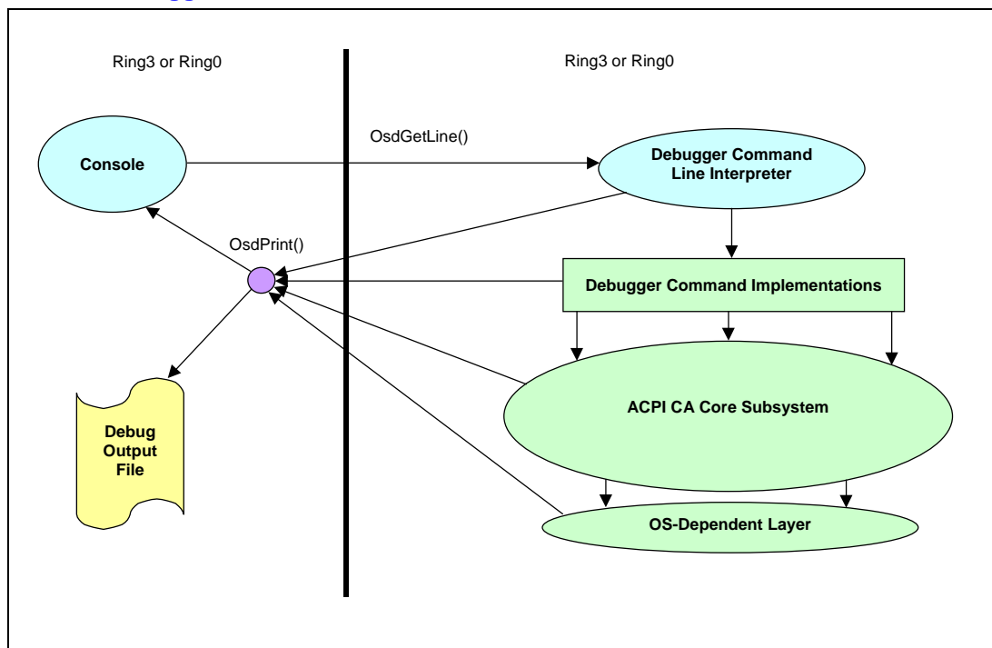
Figure 9. ACPICA Debugger Architecture
